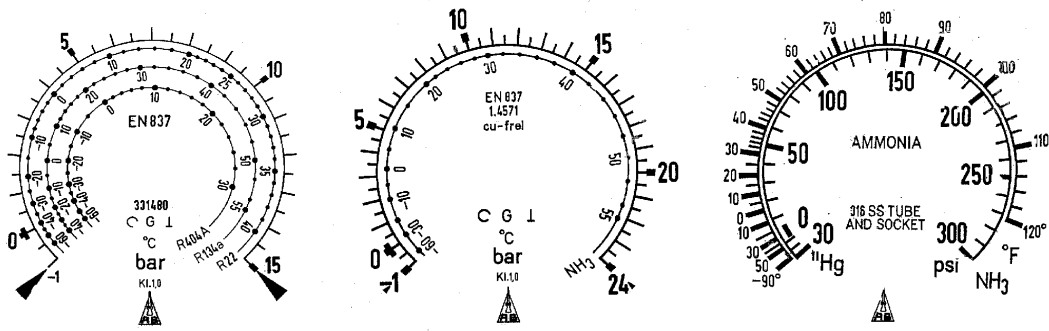
Samples of pressure/temperature dials
