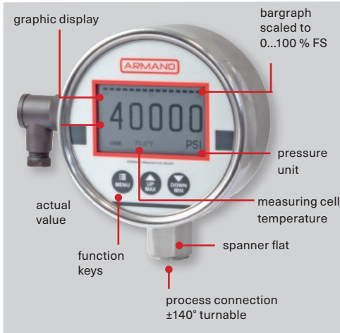
Figure 3.3-1: components
