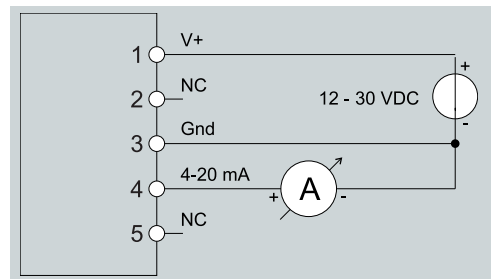
Figure 5.2-2: wiring diagram
