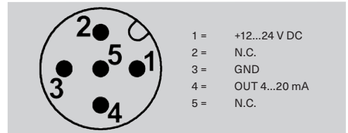
Figure 5.2-1: pin assignment
